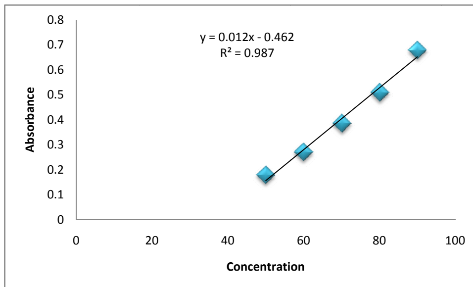
Fig 3 Calibration curve of saxagliptine
