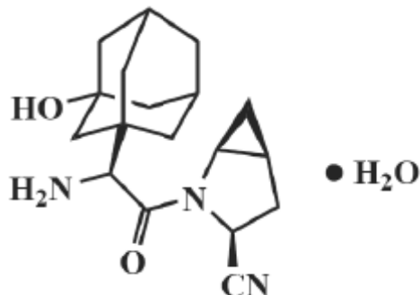
Fig 1 Structure of saxigliptine
