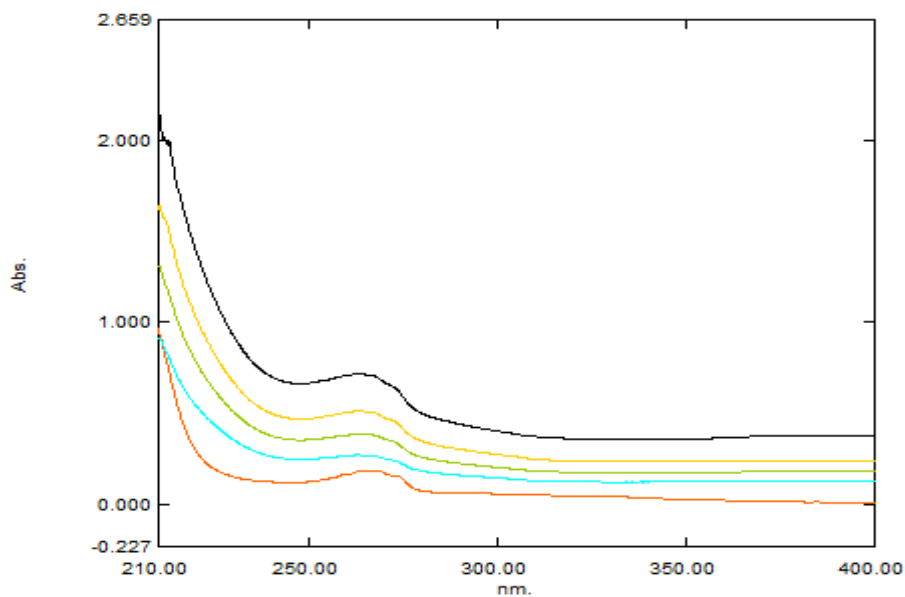
Fig 2 UV spectra of Saxagliptine
